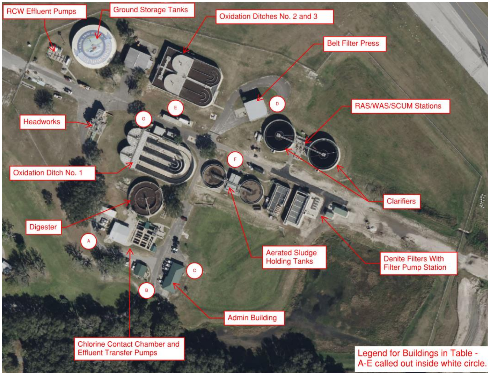
FIGURE 1 CITY OF ZEPHYRHILLS AWT FACILITY SITE LAYOUT
